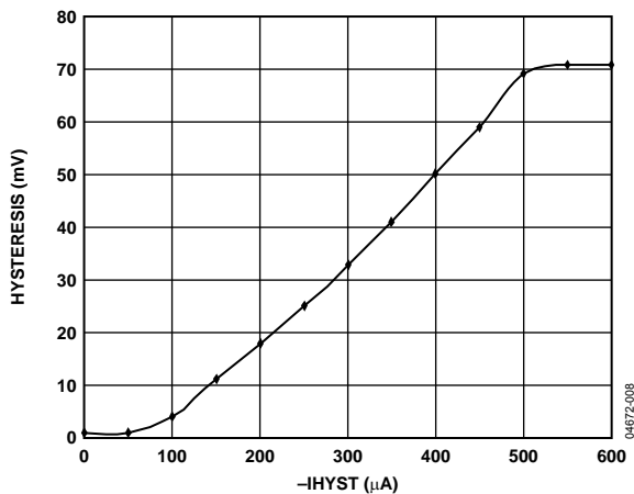
Figure 8. Hysteresis vs. -IHYS
