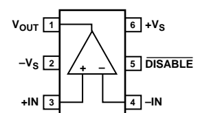
Figure 2. SC70-6 (KS)
