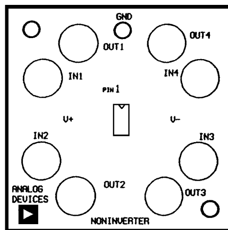
Figure 22. Silkscreen
