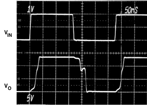
Figure 33. 50% Overload Recovery, Gain = +10, (R F = 300 Ω, R L = 1 kΩ, V S = ±7.5 V)
