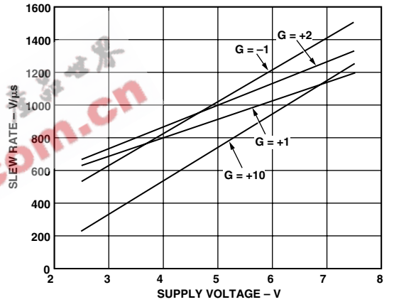
Figure 22. Maximum Slew Rate vs. Supply Voltage
