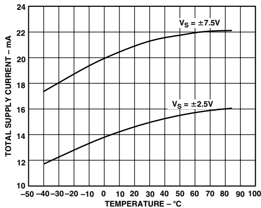
Figure 8. Total Supply Current vs. Temperature
