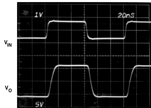
Figure 2. Output Swing Voltage, R_L = 150 \Omega ; V_S = \pm 7.5 V, G = +10
