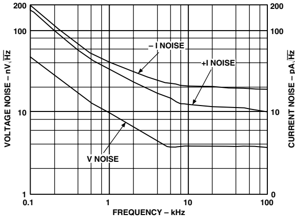
Figure 12. Input Current and Voltage Noise vs. Frequency
