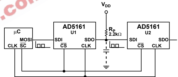
Figure 42. Daisy-Chain Configuration
