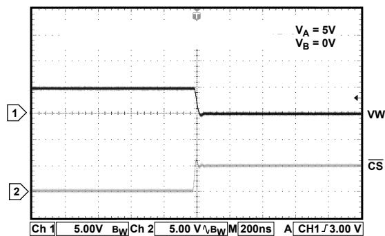
Figure 26. Large Signal Settling Time, Code 0xFF-0x00
