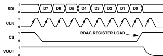
Figure 36. AD5161 SPI Interface Timing Diagram ( V_A = 5\text{ V} , V_B = 0\text{ V} , V_W = V_{OUT} )
