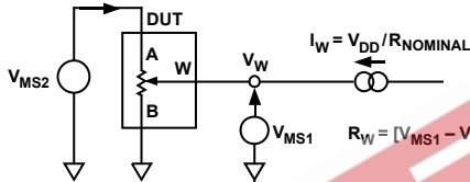
Figure 29. Test Circuit for Wiper Resistance
