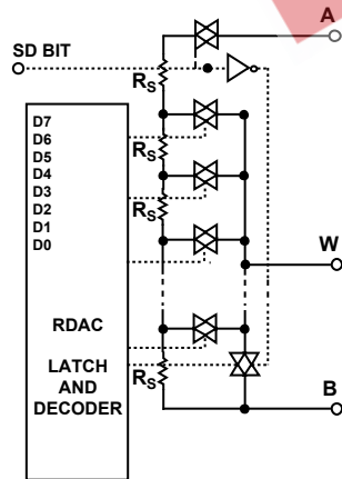
Figure 41. AD5161 Equivalent RDAC Circuit
