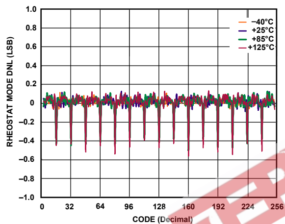
Figure 10. R-DNL vs. Code, V_{DD} = 5\text{ V}
