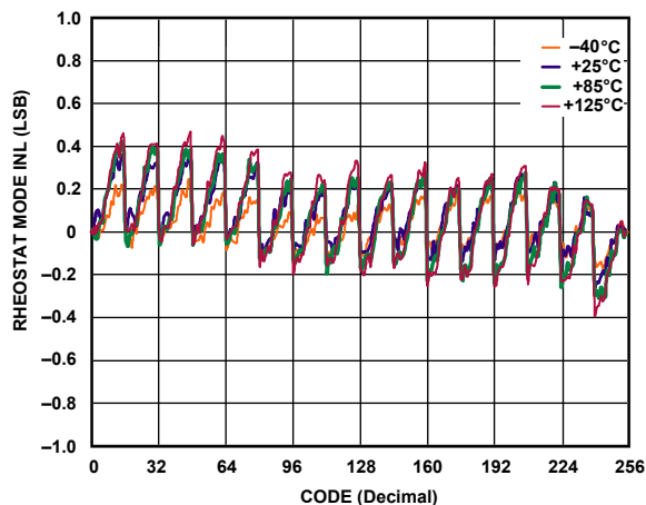
Figure 9. R-INL vs. Code, V_{DD} = 5\text{ V}
