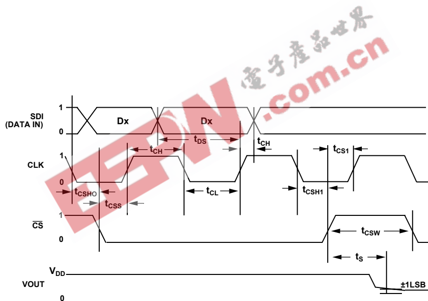
Figure 37. SPI Interface Detailed Timing Diagram ( V_A = 5\text{ V} , V_B = 0\text{ V} , V_W = V_{OUT} )
