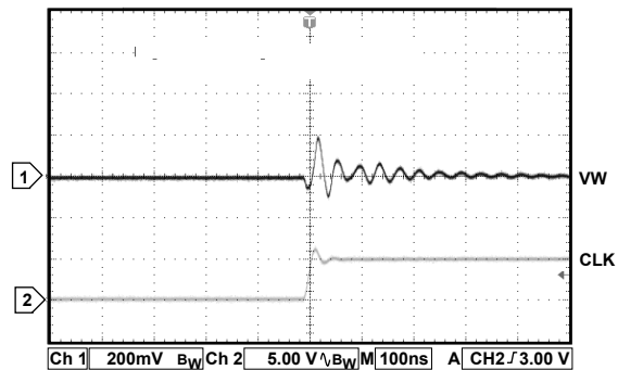
Figure 24. Digital Feedthrough
