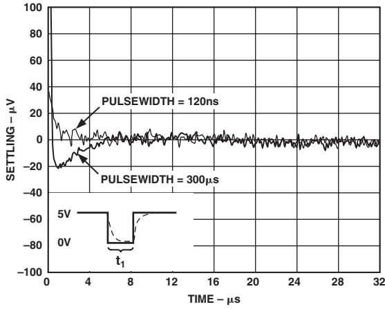
TPC 31. Long-Term Settling, 0 V to 5 V, V_S = \pm 12\text{ V} , G = +13
