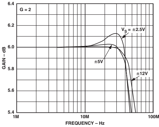
TPC 13. 0.1 dB Flatness vs. Frequency and Supply, V_{OUT} = 1\text{ V p-p} , R_L = 150\ \Omega , Noninverting. See Test Circuit 2.
