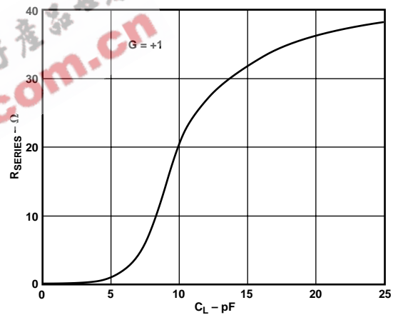
Figure 45. Recommended R_{SERIES} vs. Capacitive Load
