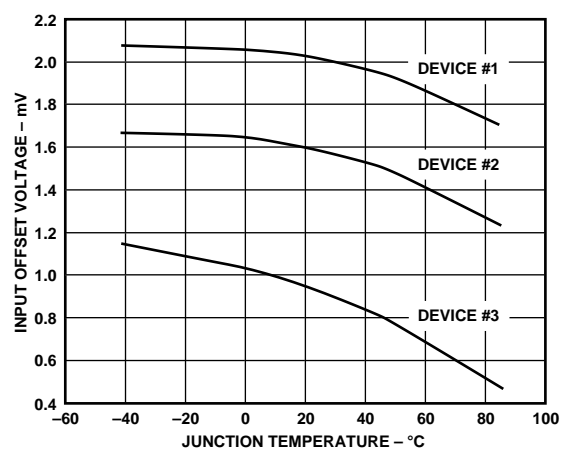
Figure 25. Input Offset vs. Temperature
