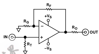
Noninverting Configuration
