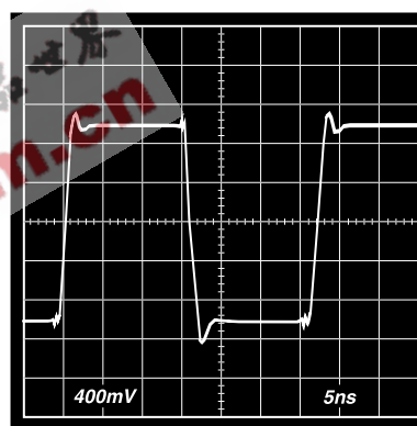
Figure 38. 2 V Step Response, G = -1
