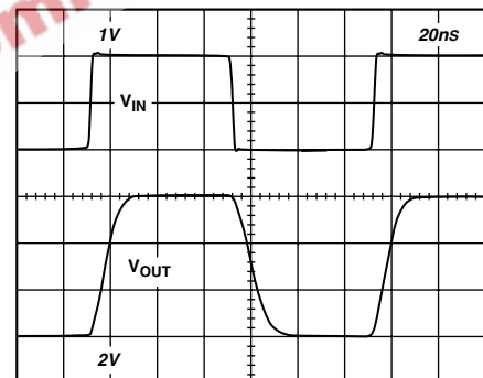
Figure 4. Pulse Response Driving a Large Load Capacitance, C_L = 300 \text{ pF} , G = +3 , R_{FB} = 2.32 \text{ k}\Omega , R_S = 10.5 \Omega , R_L = 1 \text{ k}\Omega , V_S = \pm 7.5 \text{ V}
