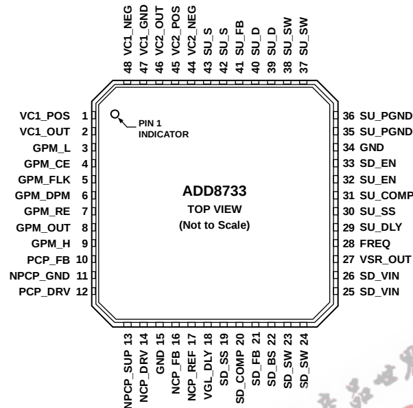
Figure 2. Pin Configuration
