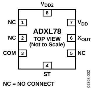
Figure 2. Pin Configuration
