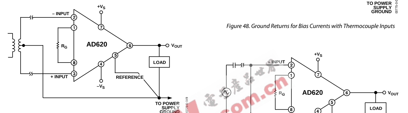
Figure 47. Ground Returns for Bias Currents with Transformer-Coupled Inputs
