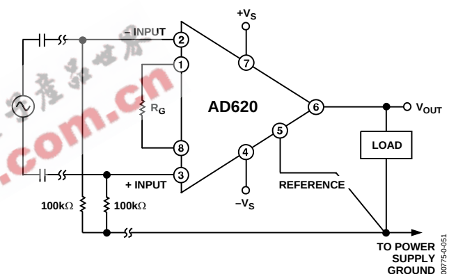
Figure 49. Ground Returns for Bias Currents with AC-Coupled Inputs
