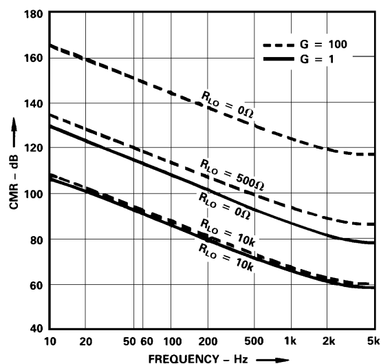
Figure 10a. AD204
