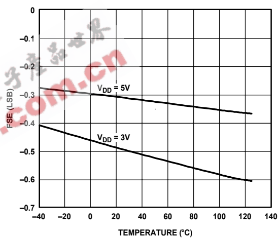
Figure 9. Full-Scale Error
