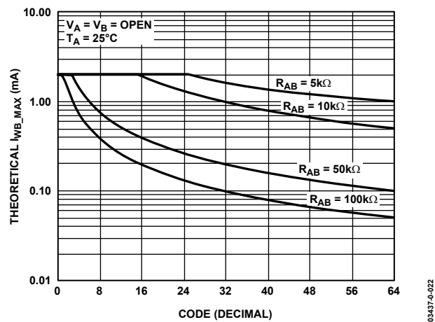
Figure 23. I_{WB\_max} vs. Code
