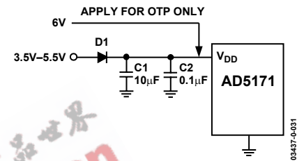
Figure 31. Isolating the 6 V OPT Supply from the 3.5V to 5.5 V Normal Operating Supply. The 6 V supply must be removed once OTP is complete.
