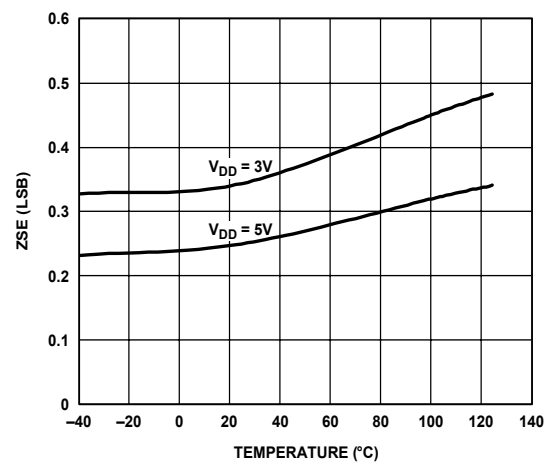
Figure 10. Zero-Scale Error
