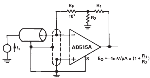
Figure 13. Picoampere to Voltage Converter with Gain
