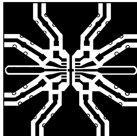
Figure 20. Component Side
