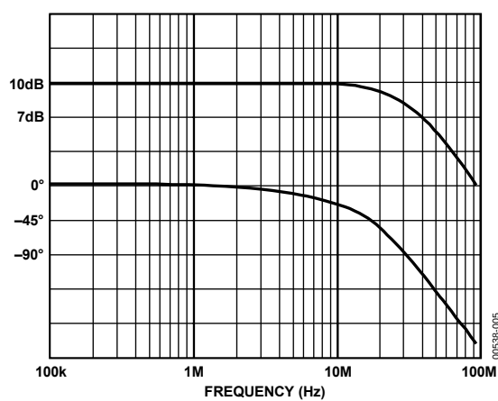
Figure 5. AD602 Frequency and Phase Response vs. Gain
