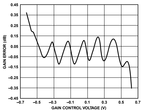
Figure 3. Gain Error vs. Gain Control Voltage
