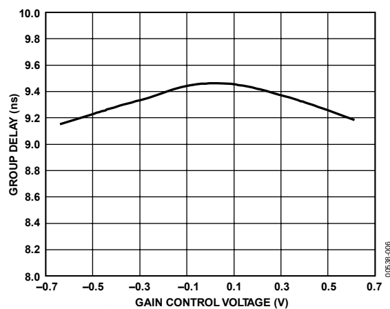
Figure 6. AD600 and AD602 Typical Group Delay vs. V_G
