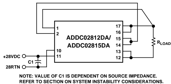
Figure 29. Typical Connections for Providing 24 V Output/30 V Output from ADC02812DA/ADDC02815DA Respectively
