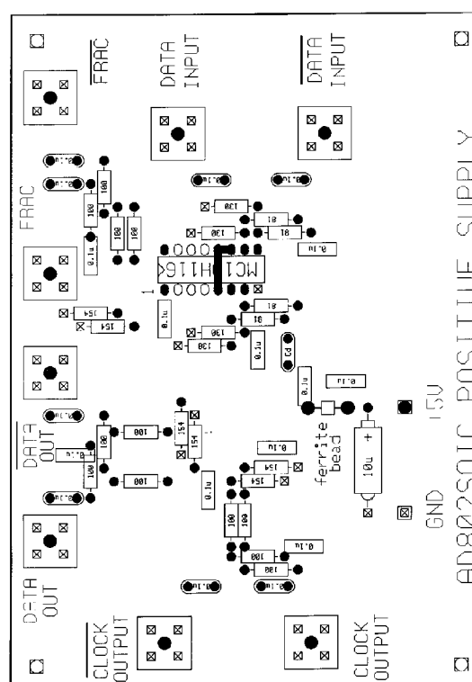
Figure 30. Positive Supply Configuration: Solder Side
