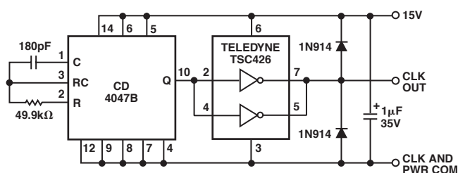
Figure 4. Clock Driver
