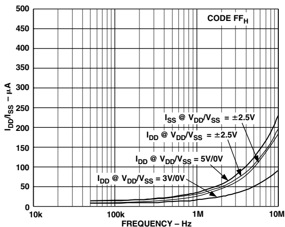
TPC 13. AD5200 10 k \Omega Supply Current vs. Clock Frequency
