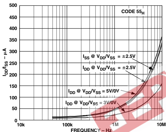
TPC 14. AD5200 10 k \Omega Supply Current vs. Clock Frequency
