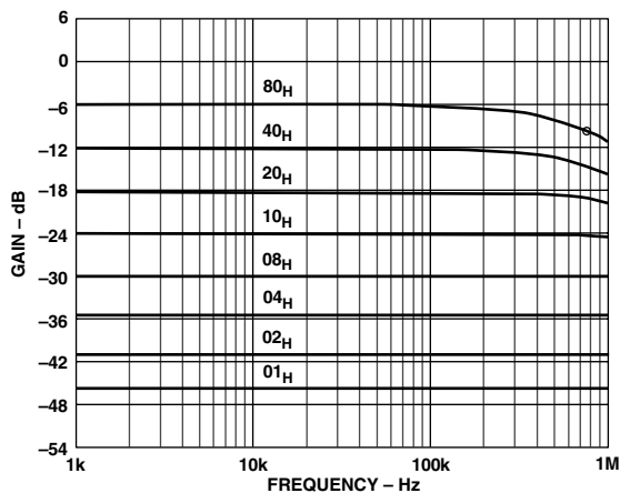
TPC 16. AD5200 10 k \Omega Gain vs. Frequency vs. Code
