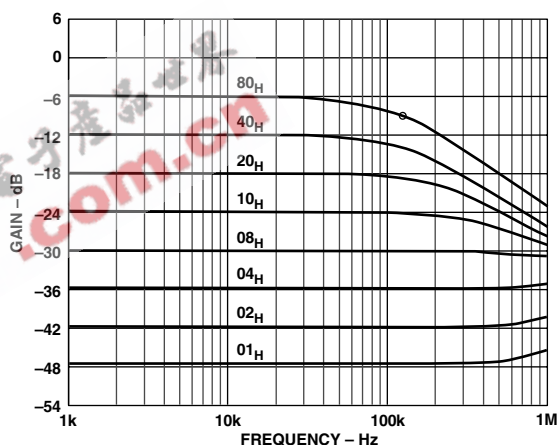
TPC 17. AD5200 50 k \Omega Gain vs. Frequency vs. Code
