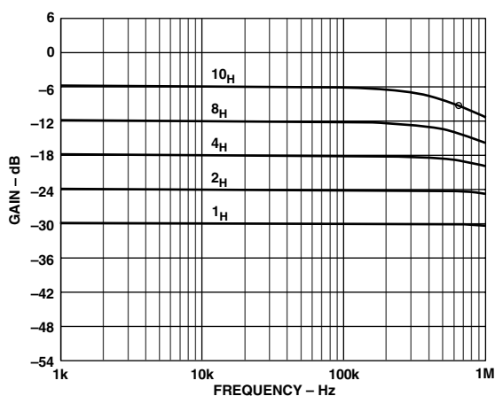
TPC 18. AD5201 10 k \Omega Gain vs. Frequency vs. Code
