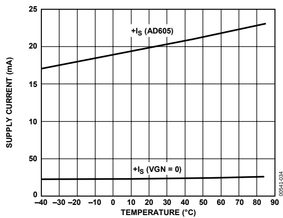
Figure 33. Supply Current (One Channel) vs. Temperature
