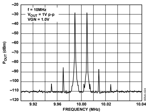
Figure 23. Intermodulation Distortion
