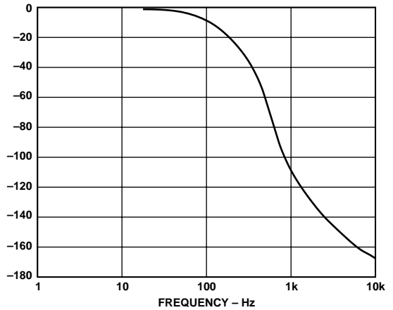
Figure 19. AD2S90 Phase Plot
