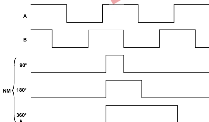
Figure 2. Incremental Encoder
