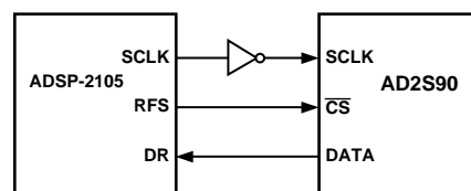
Figure 10. ADSP-2105/AD2S90 Serial Interface
