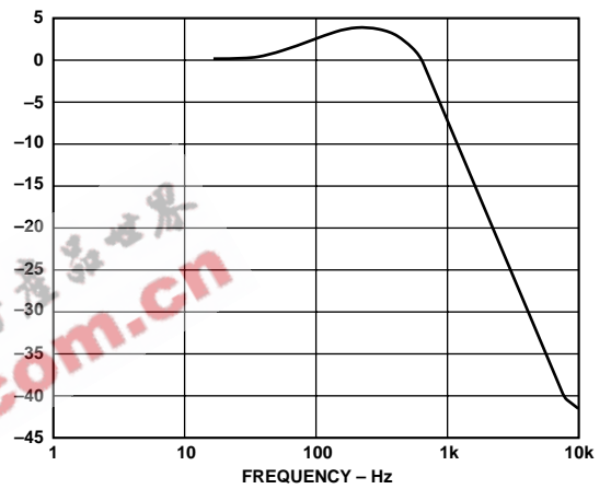
Figure 18. AD2S90 Gain Plot
