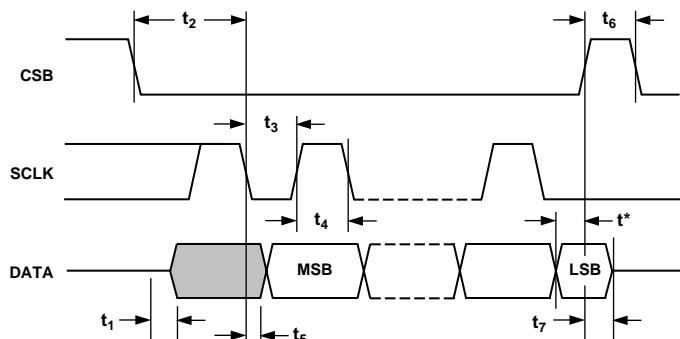
Figure 1. Serial Interface
