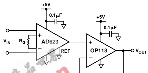
Figure 48. Output Buffering
