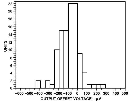
Figure 5. Typical Distribution of Output Offset Voltage, V_S = +5 , Single Supply, V_{REF} = -0.125 V; Package Option N-8, SO-8
