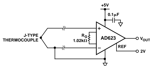
Figure 50. Amplifying Bipolar Signals with Low Common-Mode Voltage
