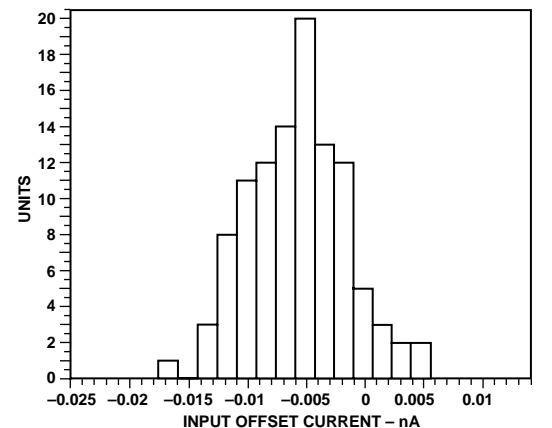
Figure 7. Typical Distribution for Input Offset Current, V_S = +5 , Single Supply, V_{REF} = -0.125 V; Package Option N-8, SO-8
