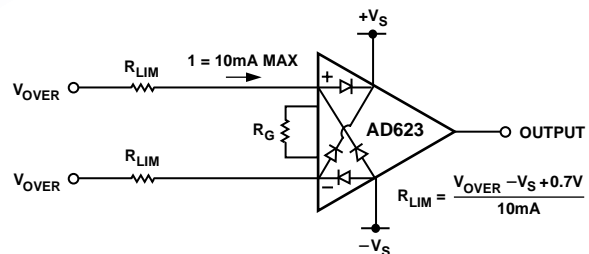
Figure 42. Input Protection
