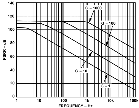
Figure 23. Positive PSRR vs. Frequency, \pm 5 V_S
