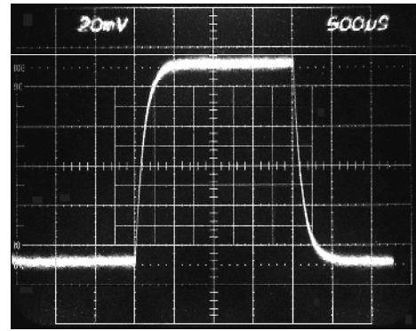
Figure 35. Small Signal Pulse Response, G = 1000 , R_L = 10\text{ k}\Omega , C_L = 100\text{ pF}
