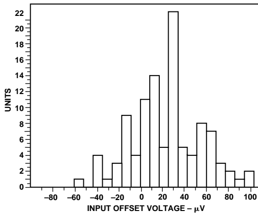
Figure 4. Typical Distribution of Input Offset Voltage, V_S = +5 , Single Supply, V_{REF} = -0.125 V; Package Option N-8, SO-8
