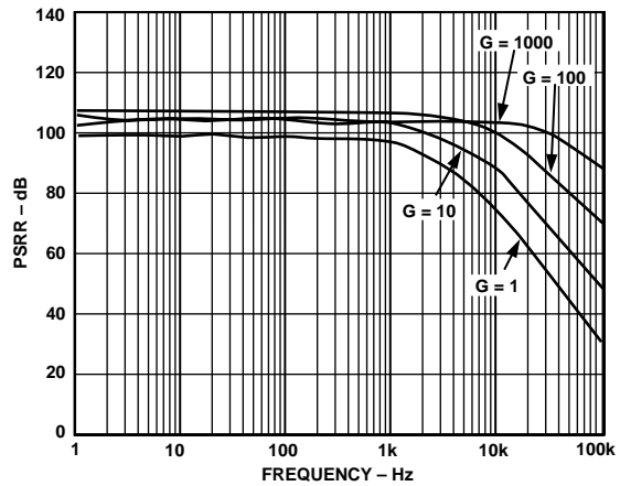
Figure 25. Negative PSRR vs. Frequency, \pm 5 V_S
