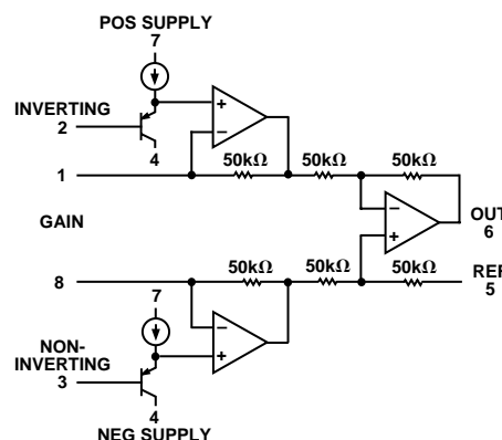
Figure 40. Simplified Schematic
