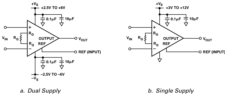
Figure 41. Basic Connections
