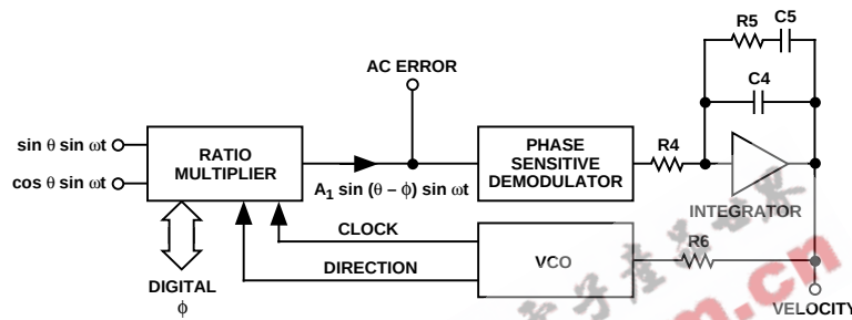
Figure 3. Functional Diagram
