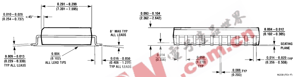
Wide-Body Small-Outline Package (M) Order Number ADC08061CIWM, or ADC08062CIWM NS Package Number M20B
