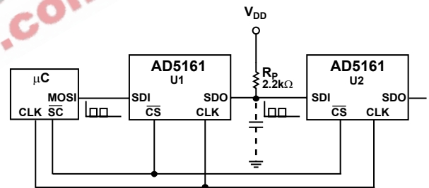
Figure 42. Daisy-Chain Configuration
