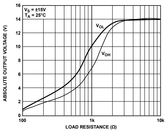
Figure 15. Absolute Output Voltage vs. Load Resistance
