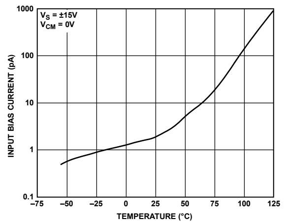
Figure 8. AD8682 Input Bias Current vs. Temperature
