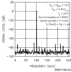
Spectral Response with 100 kHz Sine Wave Input
