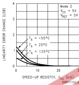
Linearity Change vs Speed-Up Resistor
