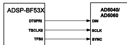
Figure 2X. AD5040/AD5060 to Blackfin ADSP-BF53X Interface
