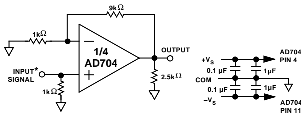
ALL 4 AMPLIFIERS ARE CONNECTED AS SHOWN
