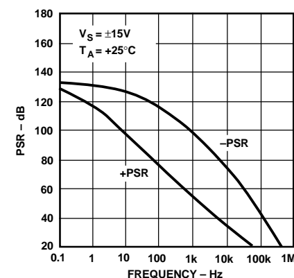
Figure 17. Power Supply Rejection vs. Frequency
