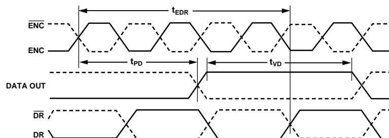
Figure 4. Highlighted Timing Diagram
