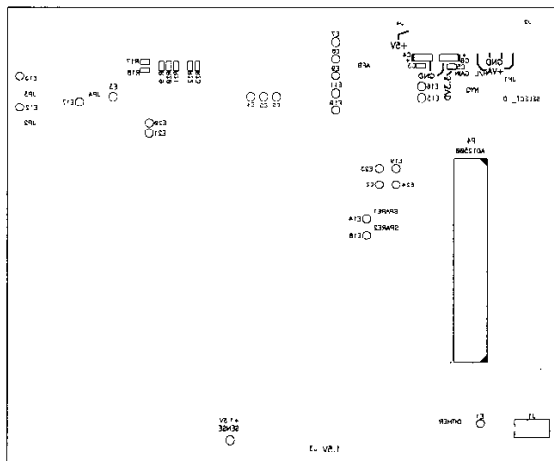
Figure 34. Bottom Silkscreen
