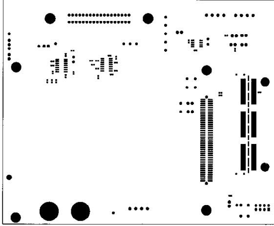
Figure 32. Top Mask
