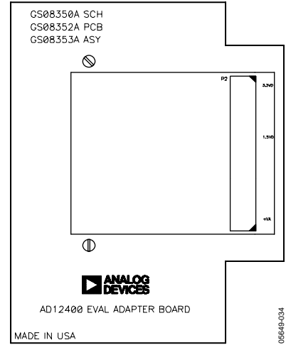
Figure 35. Evaluation Adapter Board, Top Silkscreen
