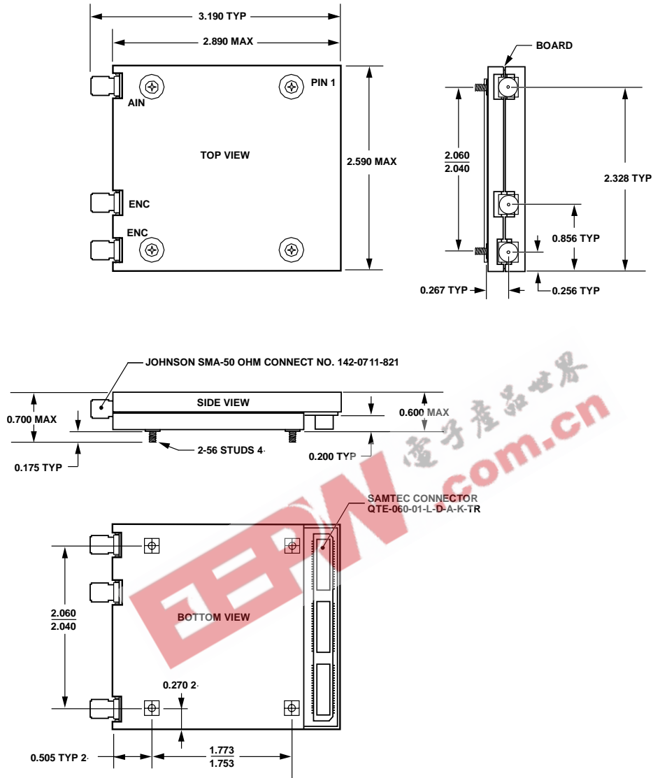
Figure 39. Non-Hermetic Hybrid—Surface-Mounted Parts (WS-Suffix) Dimensions shown in inches Tolerances: 0.xxx = \pm 5 mils
