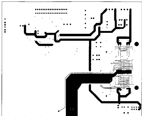
Figure 26. Power Plane 1
