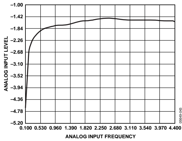
Figure 18. Low Frequency Gain Flatness
