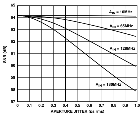
Figure 21. SNR vs. Aperture Jitter
