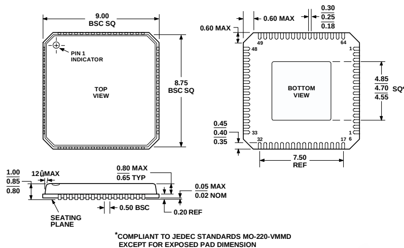
Figure 20. 64-Lead Frame Chip Scale Package (LFCSF)
