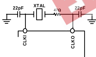
Figure 17. Crystal Connection
