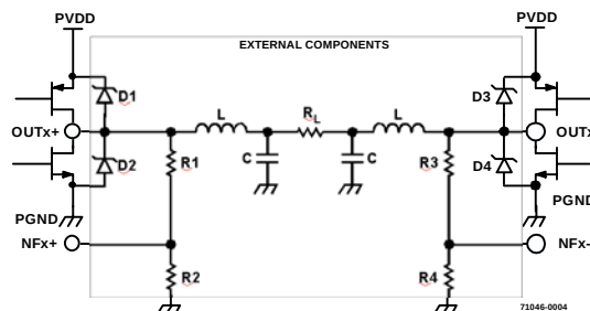
Figure 16. H-Bridge Configuration
