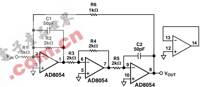
Figure 42. 2 MHz Biquad Bandpass Filter Using AD8054
