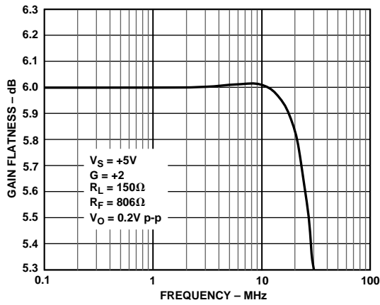
Figure 9. AD8051/AD8052 0.1 dB Gain Flatness vs. Frequency; G = +2
