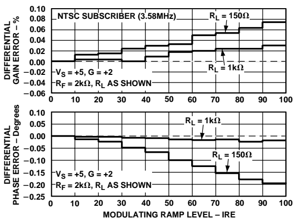
Figure 17. AD8051/AD8052 Differential Gain and Phase Errors
