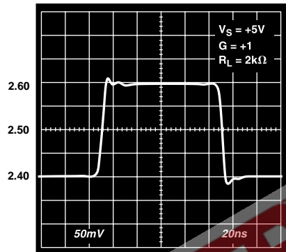
Figure 31. AD8051/AD8052 200 mV Step Response; V_S = +5 \text{ V} , G = +1
