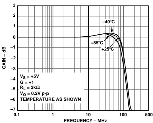
Figure 5. AD8051/AD8052 Gain vs. Frequency vs. Temperature
