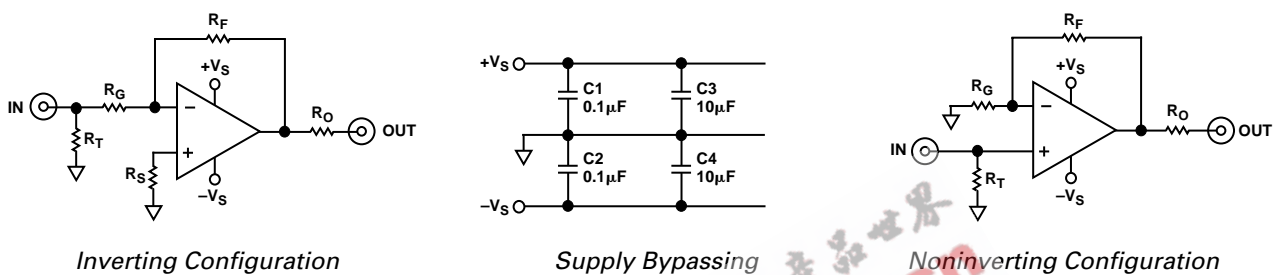
Figure 49. Inverting and Noninverting Configurations for Evaluation Boards
