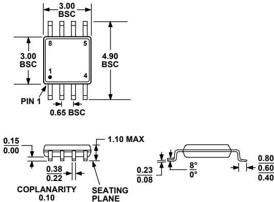
Figure 34. 8-Lead Mini Small Outline Package [MSOP] (RM-8)
