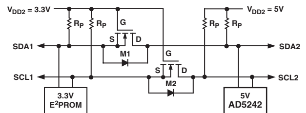
Figure 6. Level-Shift for Different Voltage Devices Operation
