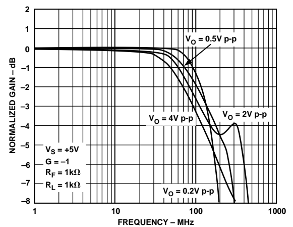
Figure 6. Bandwidth vs. Output Level—Single Supply, Gain of -1
