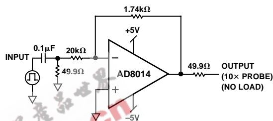
Figure 21. AD8014 as a Photodiode Preamp
