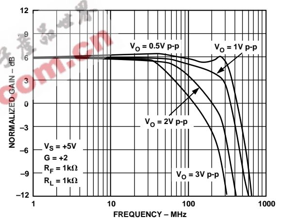
Figure 5. Bandwidth vs. Output Level—Single Supply, G = +2
