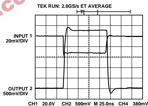
Figure 22. Pulse Response
