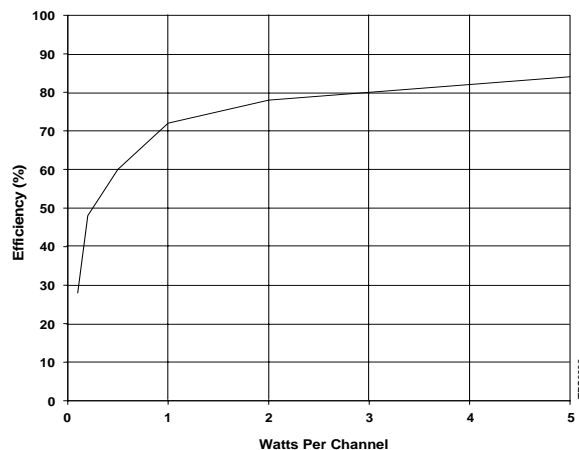
Figure 13. Efficiency vs Power
