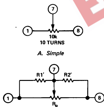
Figure 1. Nulling Circuits
