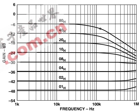
TPC 17. AD5200 50 k \Omega Gain vs. Frequency vs. Code
