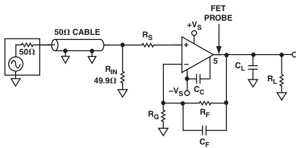
Test Circuit 2. Noninverting Gain with FET Probe
