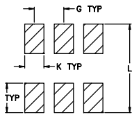
FOOT PRINT FOR PCB DESIGN
