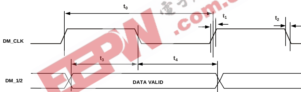
Figure 3. Uniplex Microphone Timing
