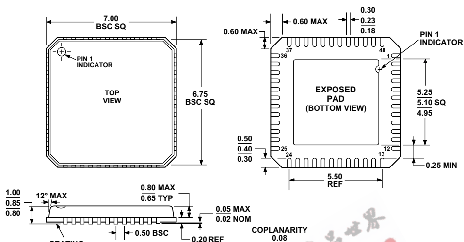
Figure 6. 48-Lead, Frame Chip Scale Package [LFCSP_VQ] 7 mm x 7 mm Body, Very Thin Quad (CP-48-1) Dimensions shown in millimeters
