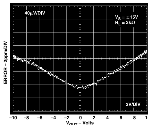
Figure 14. Gain Nonlinearity; V_S = \pm 15\text{ V} , R_L = 2\text{ k}\Omega
