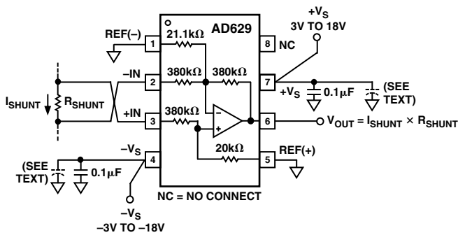
Figure 29. Basic Connections
