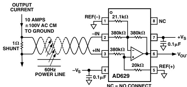
Figure 38. Error Budget Analysis Example 2. V_{IN} = 10\text{ V} Full-Scale, V_{CM} = \pm 100\text{ V} at 500\text{ Hz} , R_{SHUNT} = 1\ \Omega
