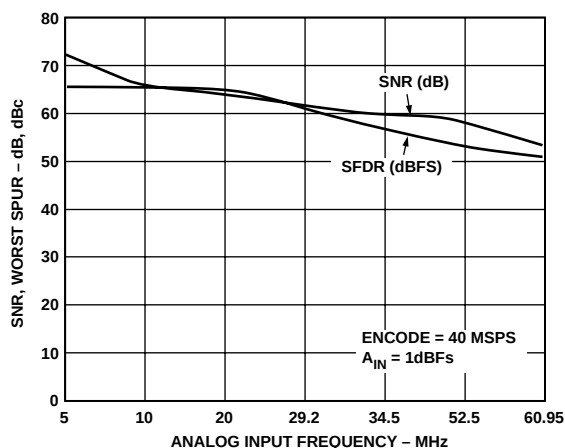
Figure 18. SNR/Harmonics to A_{IN} > \text{Nyquist MSPS}
