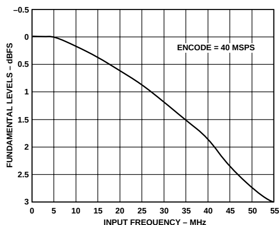
Figure 19. Gain Flatness vs. Input Frequency
