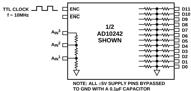
Figure 2. Equivalent Burn-In Circuit
