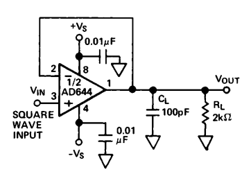
Figure 21c. Unity Gain Follower Pulse Response (Small Signal)
