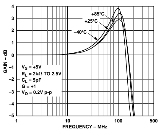
Figure 8. AD8054 Gain vs. Frequency vs. Temperature
