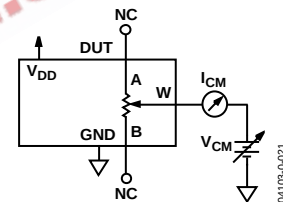
Figure 33. Test Circuit for Common-Mode Leakage Current
