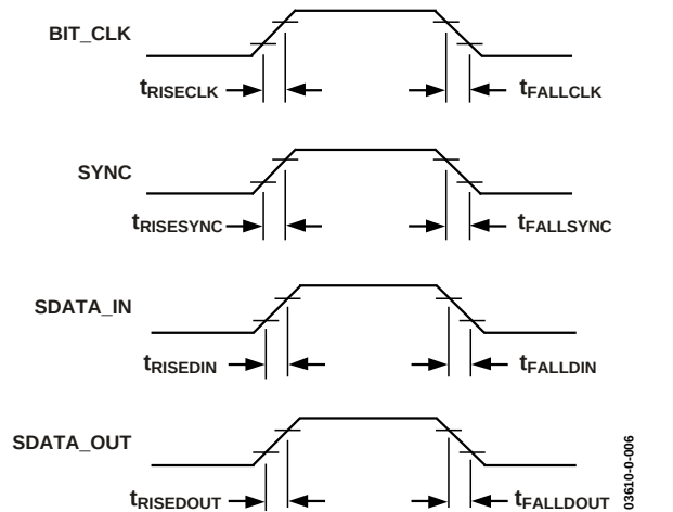
Figure 6. Signal Rise and Fall Times
