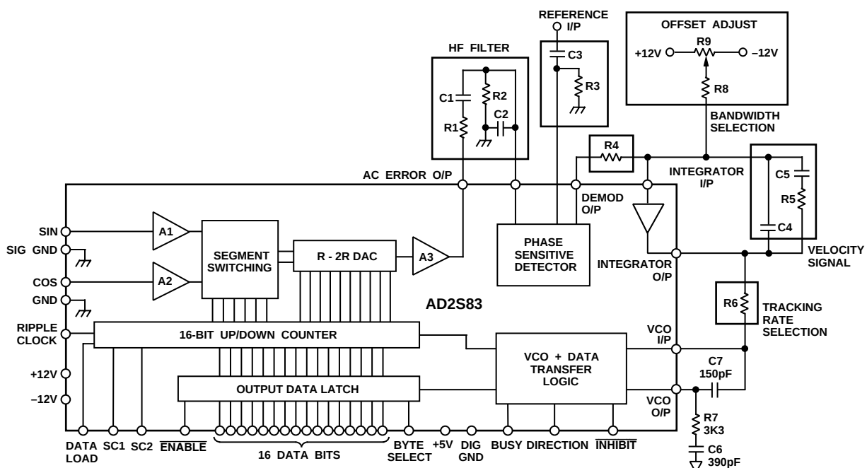
Figure 1. Connection Diagram
