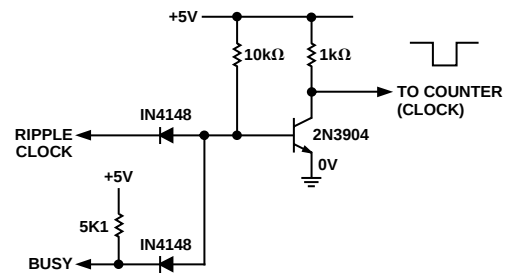
Figure 2. Diode Transistor Logic Nand Gate
