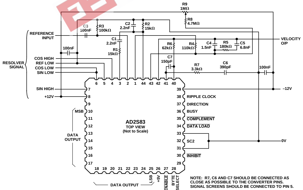
Figure 11. Typical Circuit Configuration
