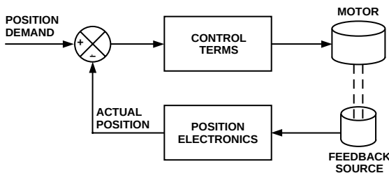
Figure 8. Position Control
