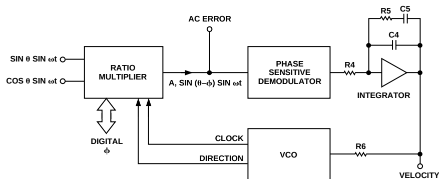
Figure 4. Functional Diagram
