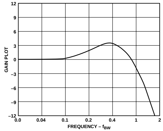
Figure 5. Gain Plot
